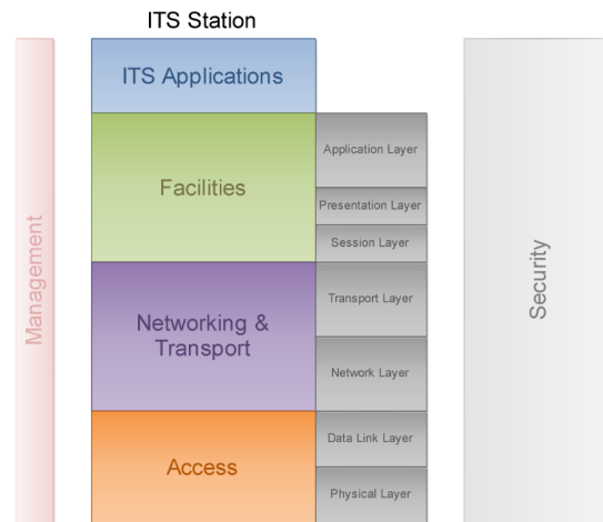
Fig. 1. The ETSI and OSI communication stacks [9].
