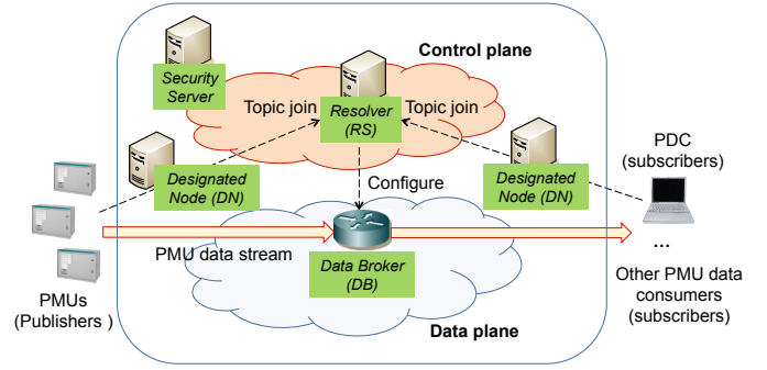
Fig. 2: C-DAX Architecture.
