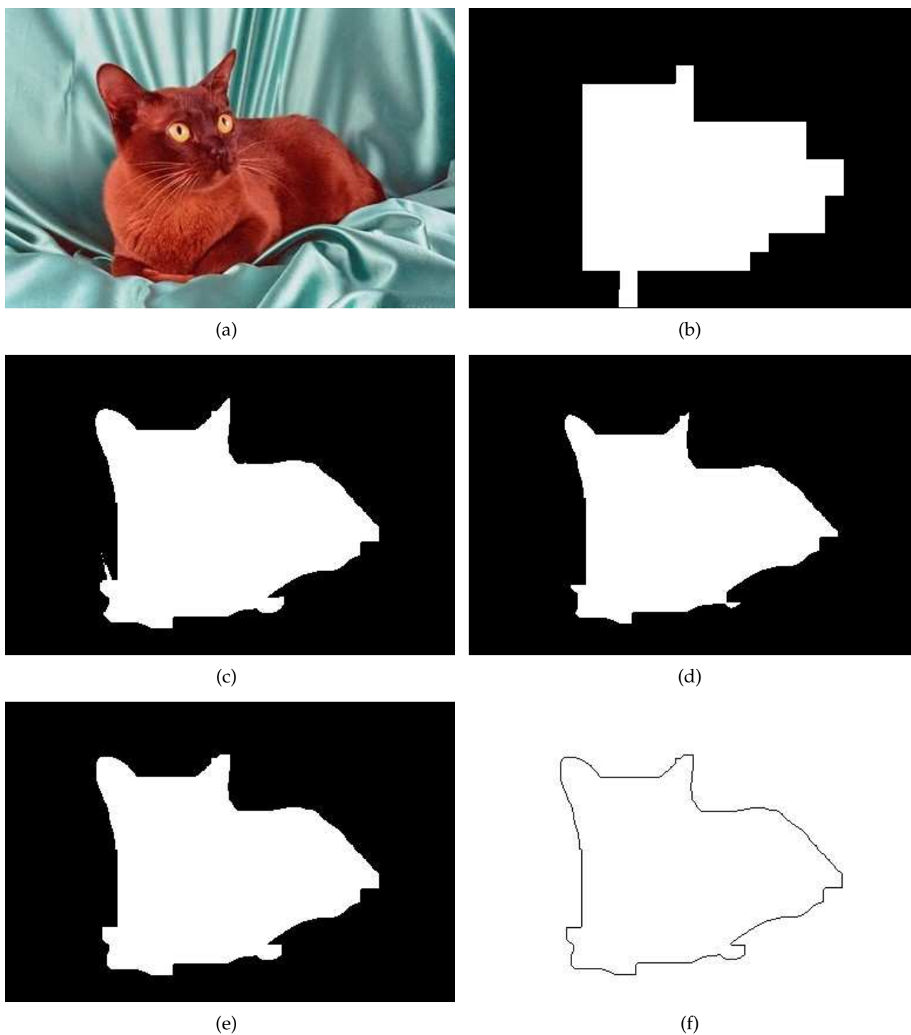
Figure B.18: (a) The original image (b) The coarse segmentation (c) The object after pixelwise classification (d) The object after erosion (e) The object after dilation (f) The final shape.
