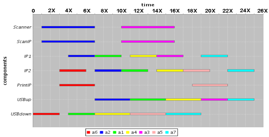
Fig. 18. Execution chart for TA model with dynamic USB behavior
