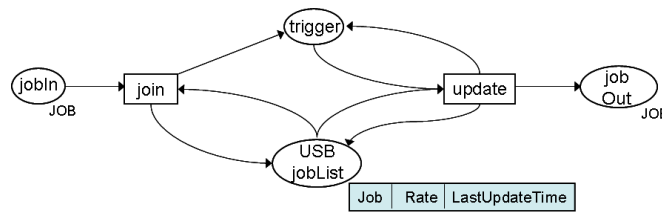
Fig. 8. CPN model for the USB
