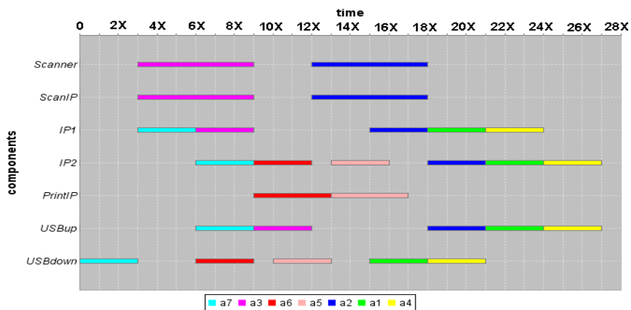
Fig. 13. Execution chart for CPN model with static USB behavior
