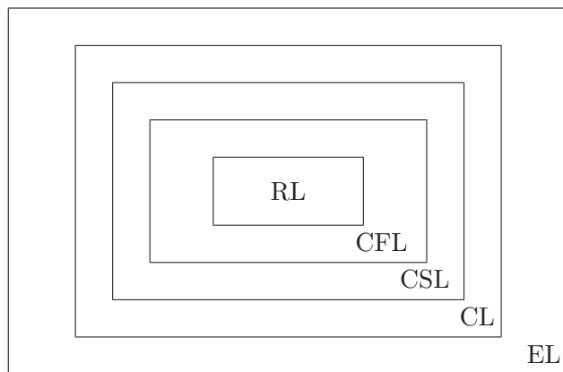
Figure 7: The Chomsky hierarchy
