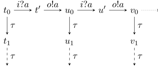
Figure 11: \mathcal{T}_{RTM}(RTM_{div})
