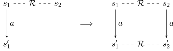
Figure 6: (Strong) bisimilarity
