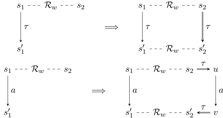
Figure 7: Weak bisimilarity
