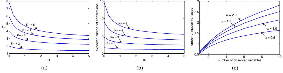
Figure 1. Empirical study of hyperparameters. Figure (a) shows the expected number of active nodes as a function of \alpha and \gamma . Figure (b) shows that once we know the expected K^+ from \alpha and \gamma , we can find the expected number of connections. Figure (c) shows the influence of \alpha (with \gamma = 1 ) on the complexity (number of hidden nodes) as function of the number of observable nodes.
