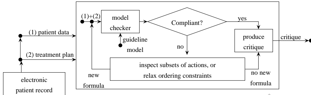
Figure 1: Critiquing approach using model checking. Given patient data and a treatment plan as input (temporal specifications), the critiquing system uses a model checker to verify consistency w.r.t. to a guideline model (state transition system) to generate a critique (empty in case of compliance).
