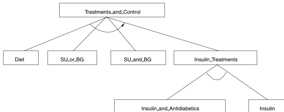
Fig. 2. Asbru plan hierarchy of the diabetes mellitus type 2 guideline.
