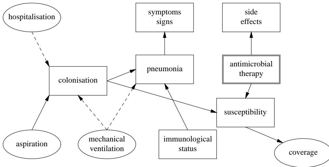
Figure 12: Global structure of the Bayesian-network model of VAP.
