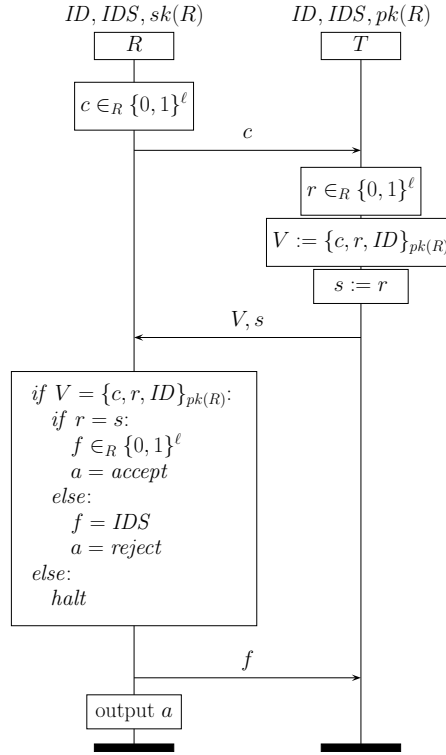
Figure 5.8: Backdoor protocol.
