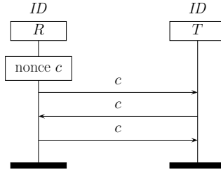
Figure 5.7: Echo protocol.
