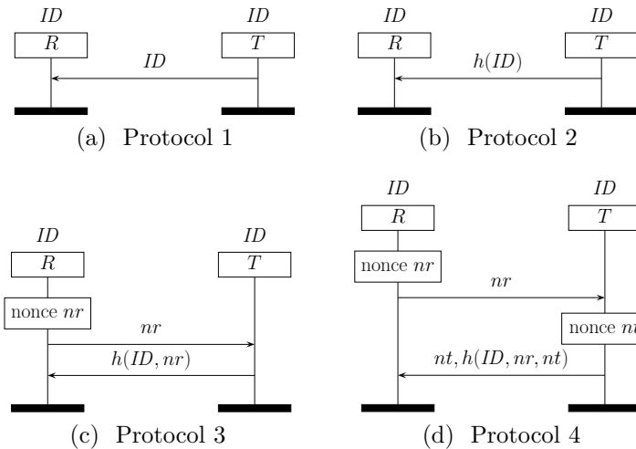
Figure 3.4: Traceable and untraceable protocols
