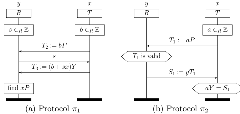
Figure 4.9: Building blocks of EC-RAC II
