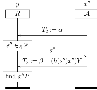
Figure 4.6: Insider attack on EC-RAC IV.
