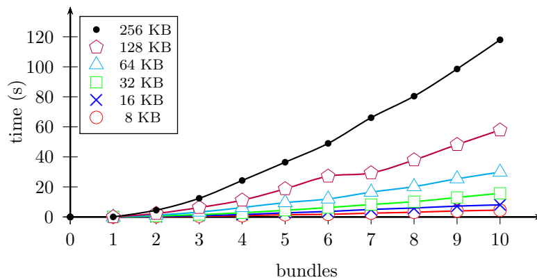
Figure 8.6: Performance
