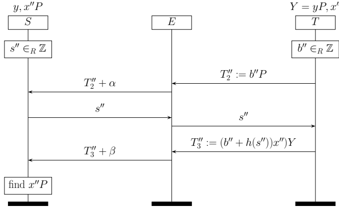
Figure 4.4: Man-in-the-middle attack on EC-RAC IV
